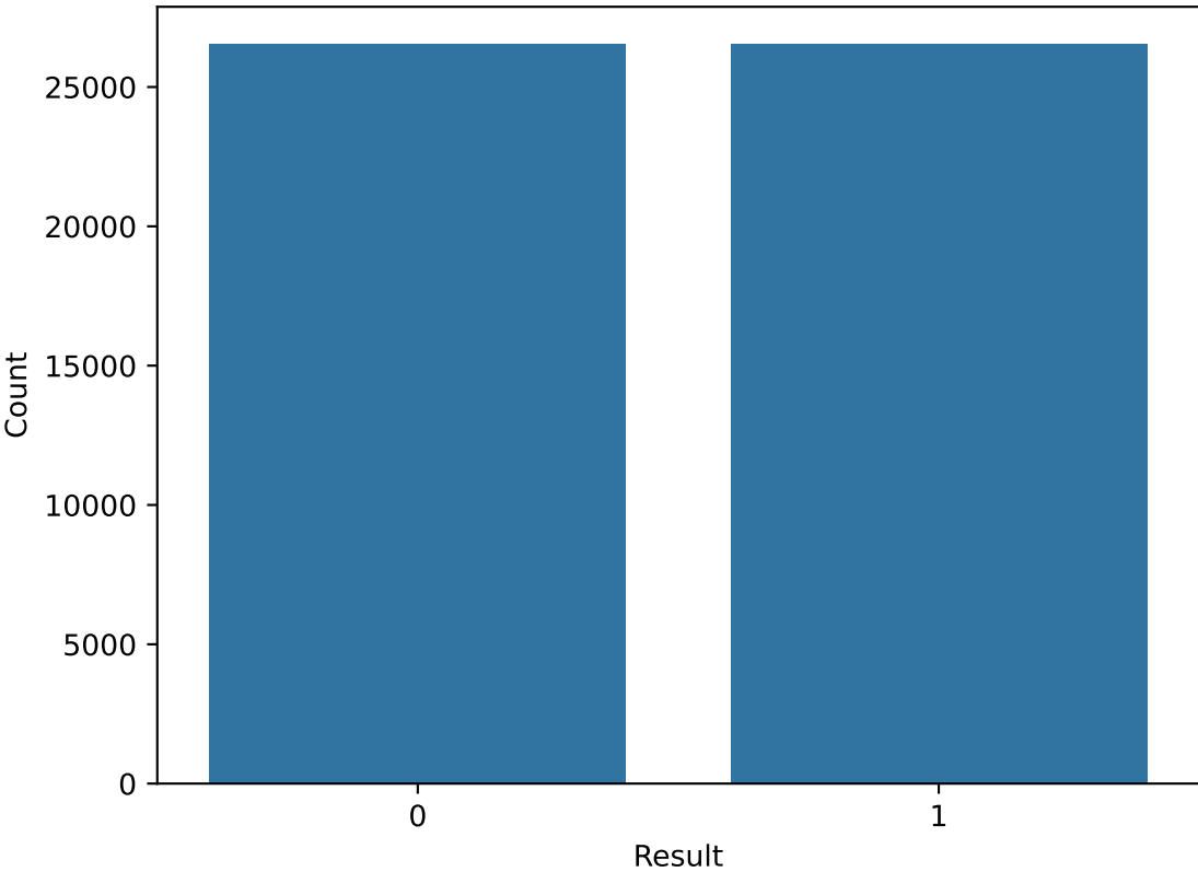
Distribution of the target variable (result)
